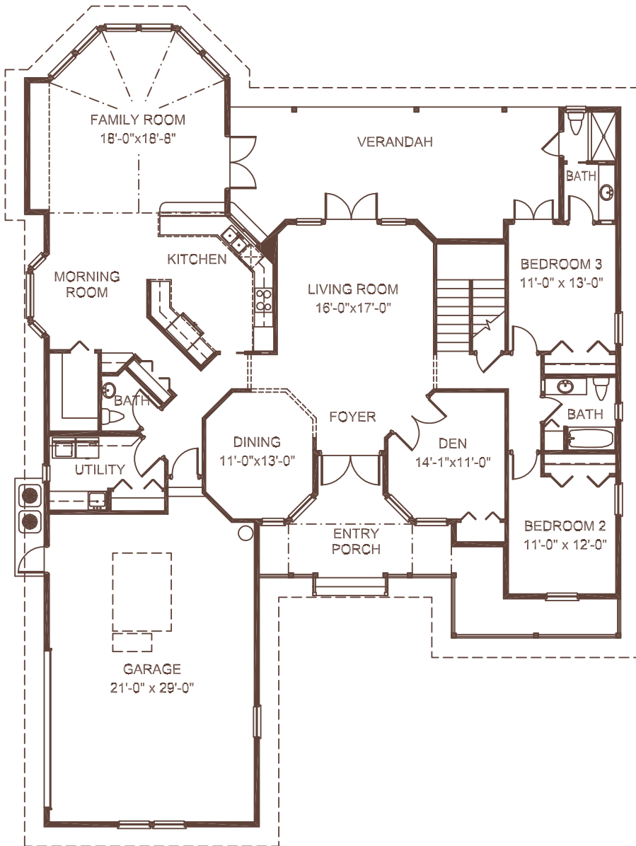
1st Floor
